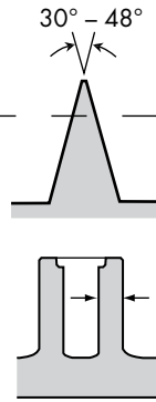
Typical Boss Design for Fastener for Plastics
