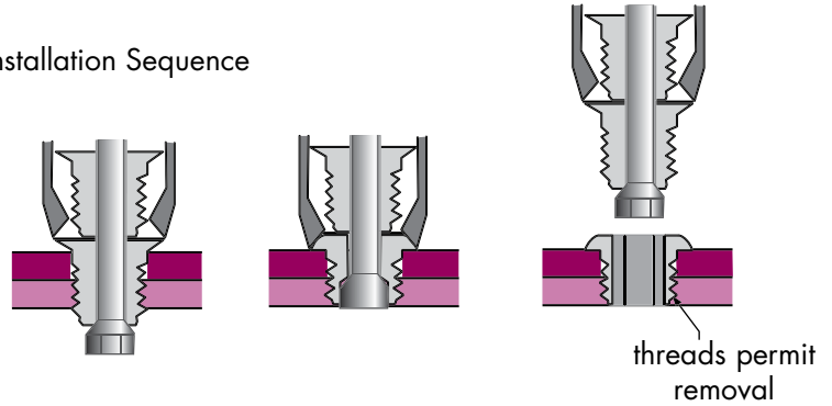
Rivscrew® Speed Fastener
