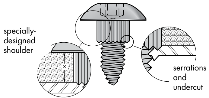
Powergrip Fastener
