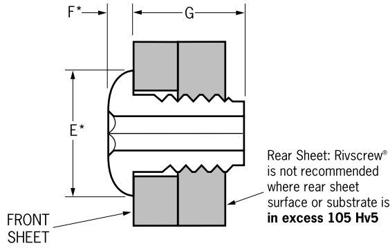
After Placement
