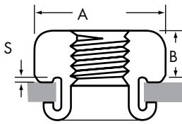
Standard Set
